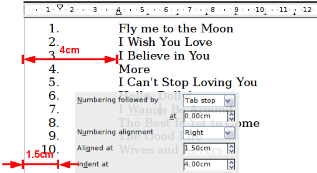
Figure 34: A numbered list of CD tracks highlighting the various elements
