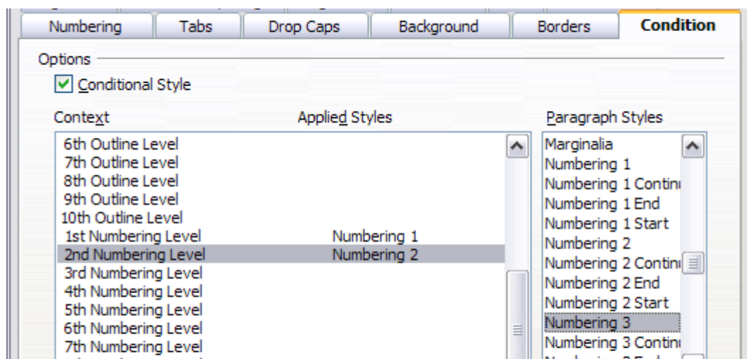
Figure 19: Condition page for paragraph styles
