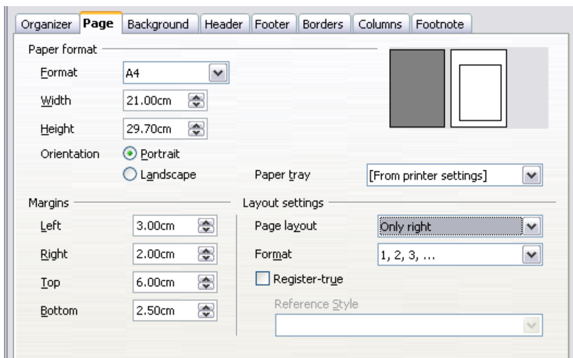
Figure 26: Setting page margins and layout for the Right Page style
